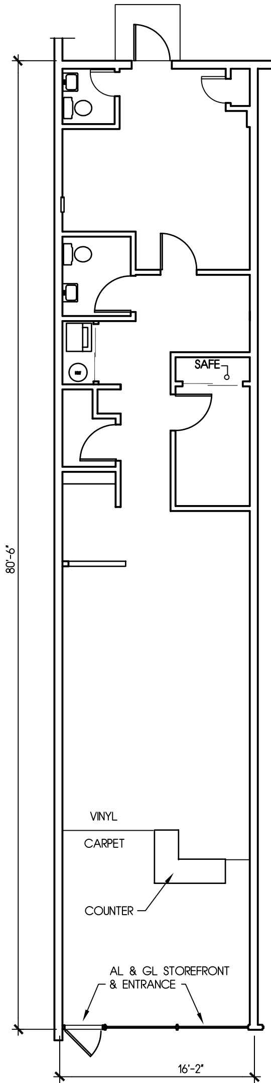
Floor Plan SCALE : 1/8" = 1'-0"
